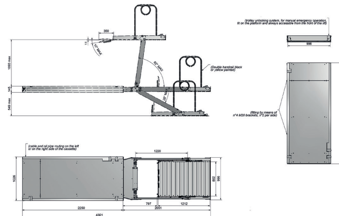
RPB 35.11 HD Dimensions in mm
