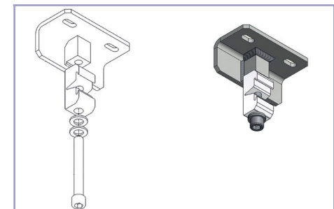
Fitting Brackets
