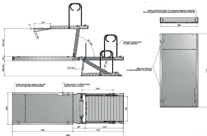
RPB 35.11 Dimensions in mm
